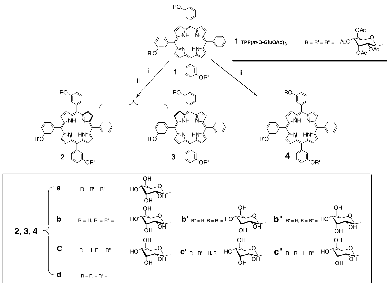
Scheme 1. Synthesis and structure of glycoconjugated chlorins and porphyrins. Reagents and conditions: (i) (a) toluene-4-sulfonohydrazide, anhydrous K 2 CO 3 , dry pyridine, 100 °C; (b) ortho -chloranil, ethyl acetate; (ii) MeONa/MeOH, 20 °C.
